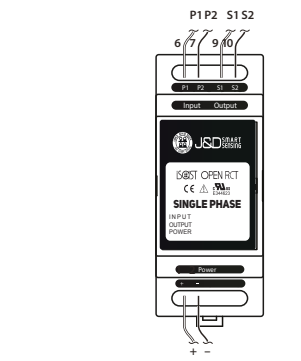
Power supply : 24V DC
